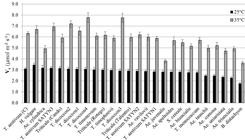
Fig. 1. Rubisco carboxylation velocity ( V_c ) at 25 °C (black bars) and 35 °C (hatched bars) in 25 Triteceae genotypes. Data organized in decreasing rank at 25 °C, except for T. aestivum cv Cadenza, which is shown on the far left-hand side for comparison.
