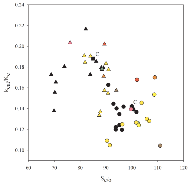
Fig. 4. The relationship between the catalytic efficiency of Rubisco at 21% O 2 ( k_{\text{cat}}/K_c , \mu\text{M s}^{-1} ) and the specificity factor ( S_{c/o} ) of Rubisco at 25 °C (circles) and 35 °C (triangles). Each colour denotes an rbcL sequence (as per Table 3) and Cadenza wheat (C, used as reference) is represented by the diamond and square at 25 and 35 °C, respectively.
