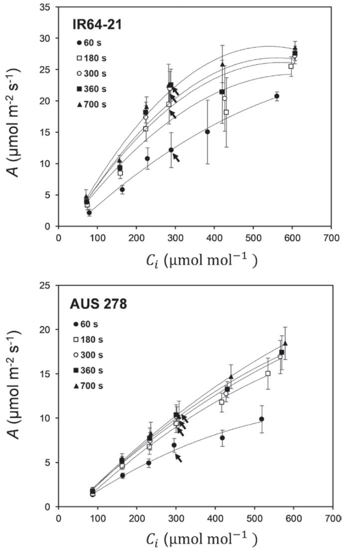
Fig. 6. The responses of leaf CO 2 assimilation ( A ) to intercellular [CO 2 ] ( C_i ) at different points in time after the beginning of photosynthetic induction for IR64-21 and AUS 278. Times after induction were: 60 s (filled circles), 180 s (open squares), 300 s (open circles), 360 s (filled squares), and 700 s (filled triangles) from the start of induction. The operating point of each curve at 400 \mu\text{mol mol}^{-1} atmospheric [CO 2 ] ( C_a ) is indicated with a black arrow. Each point is the mean ( \pm SE) of four plants of each rice accession.
