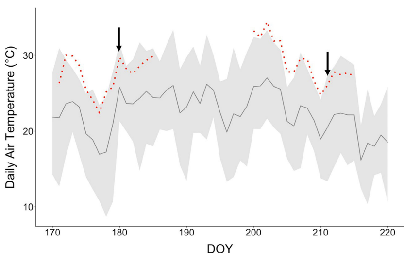
Figure 4 Daily air temperature of ambient and heated plots throughout the duration of two field-warming experiments. Solid grey line represents the mean and shaded grey regions represent the daily max-min air temperature with DOY. The average daily canopy temperature of heated plots for each experiment is plotted in the dotted red. Black arrows indicate the DOY of in situ diurnal measurements of photosynthesis in each experiment.
