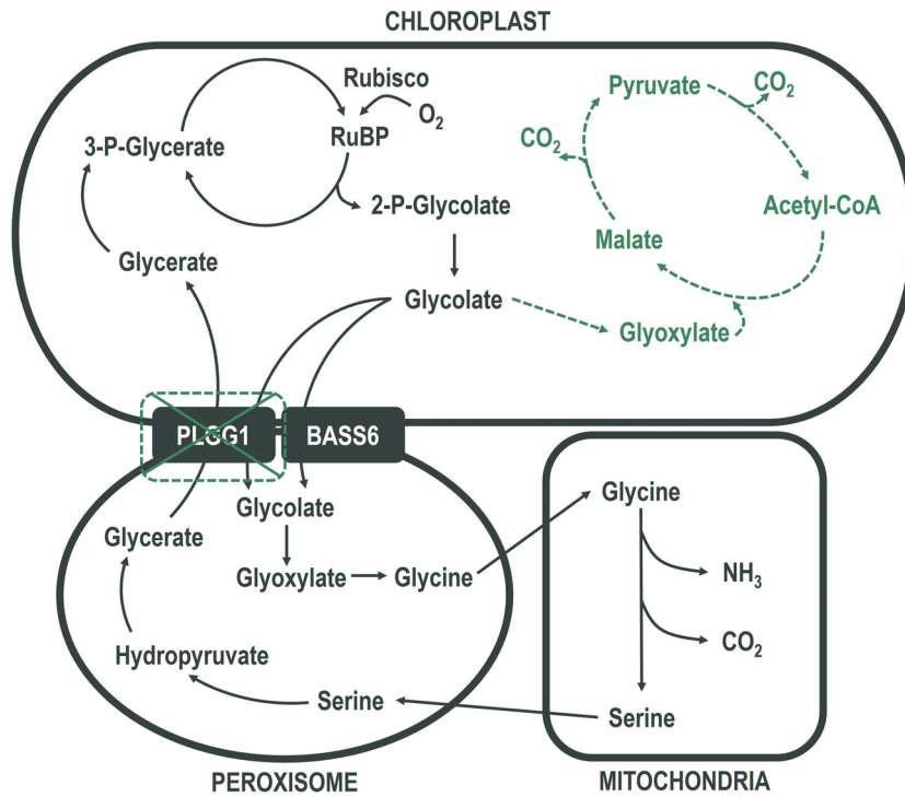
Figure 1 Pathway schematic of native and alternative photorespiration pathways. Alternative glycolate metabolism pathway (AP3) schematic. Chloroplast, peroxisome, and mitochondria based enzymatic reactions or transport steps of the native photorespiratory pathway (grey, solid lines) and AP3 (green, dashed lines) are shown. In AP3, the native glycolate-glycerate transporter PLGG1 is downregulated via RNAi suppression to increase metabolic flux through the alternative metabolic pathway.
