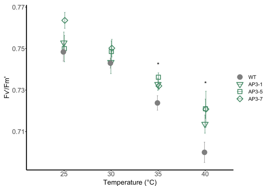
Figure 2 Photosynthetic operating efficiency ( F_v'/F_m' ) with temperature in chamber-grown AP3 and WT lines. Values are from three independently transformed AP3 construct designs with RNAi targeting the glycolate-glycerate transporter PLGG1 measured under temperature stress. Error bars indicate SEM. *Statistical difference in all AP3 lines compared to WT based on one-way repeated measures ANOVA at P < 0.05 ; n = 6 .
